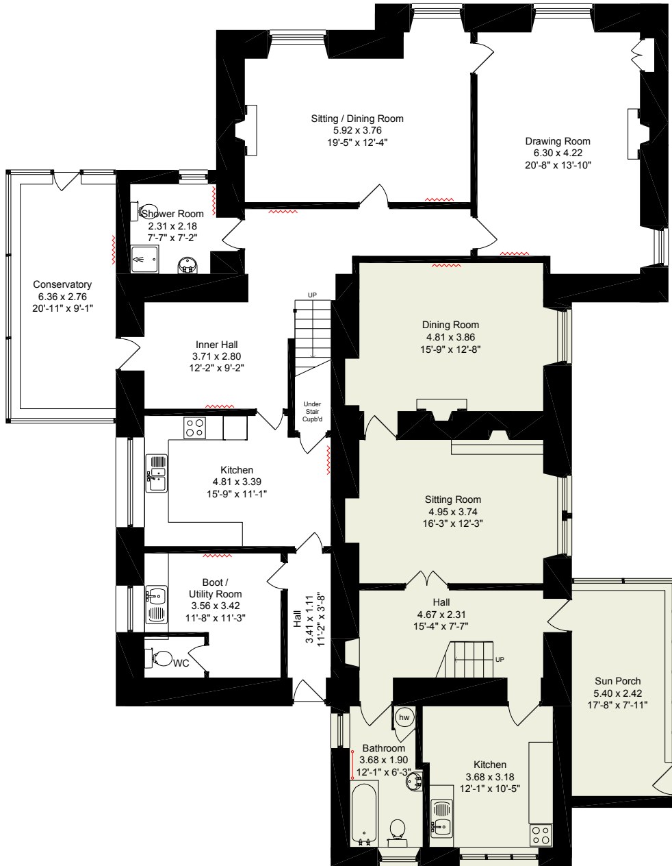
Ground Floor
